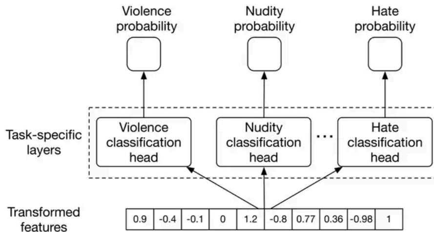
Figure 5.11: Task-specific layers
