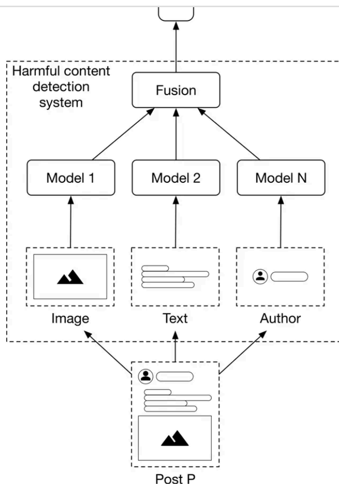
Figure 5.4: Late fusion
