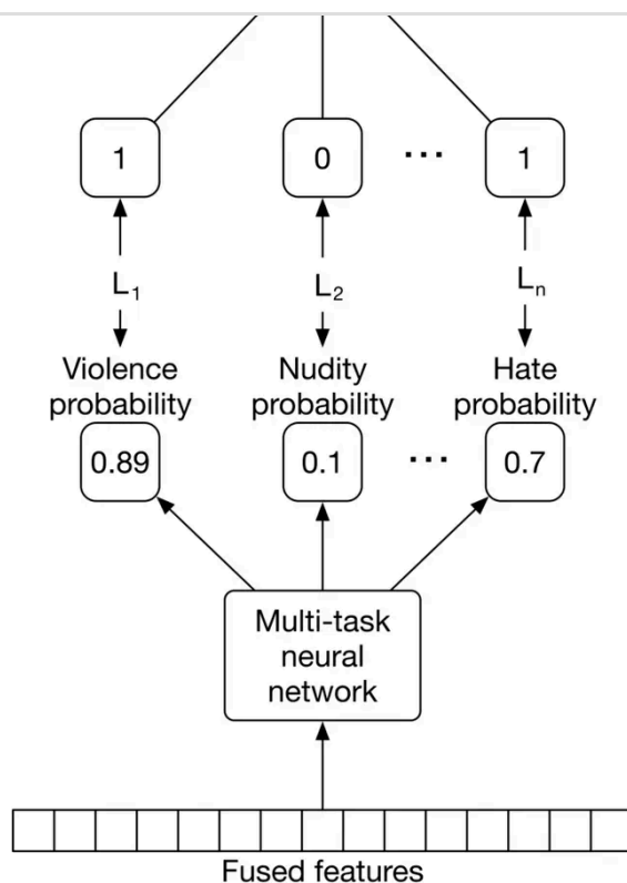
Figure 5.17: Model training
