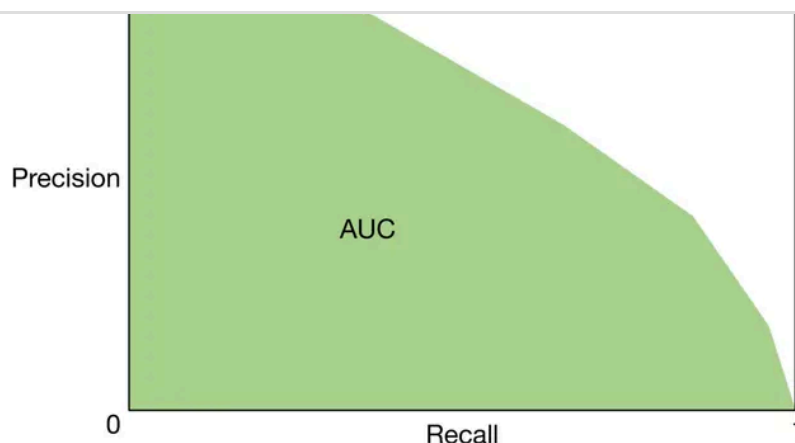
Figure 5.18: PR curve
