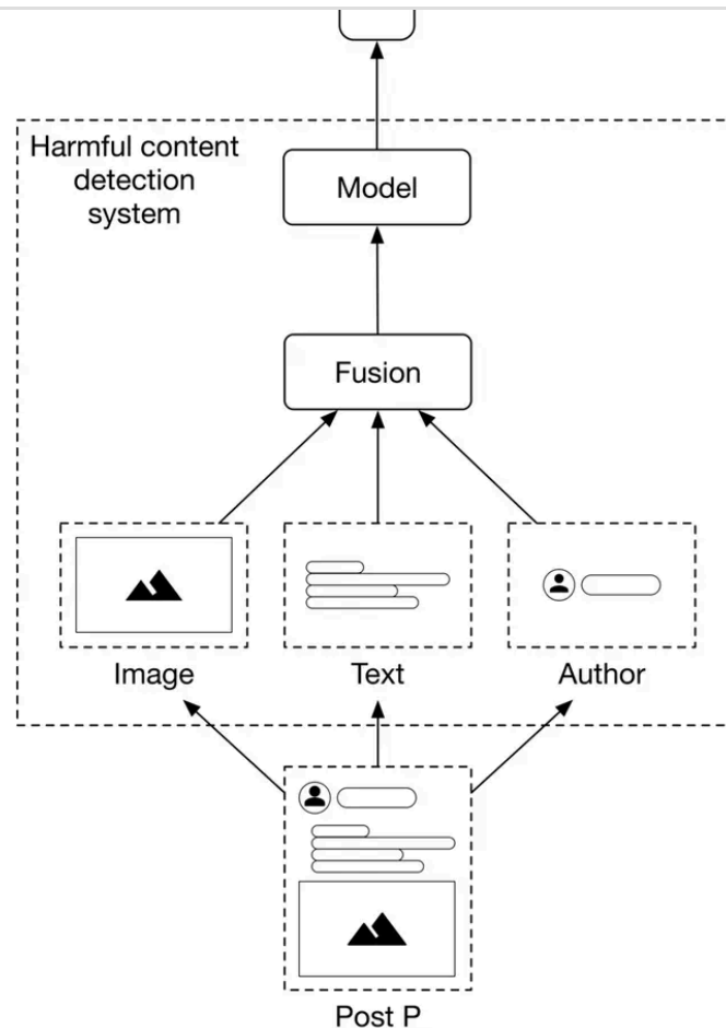
Figure 5.5: Early fusion
